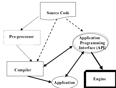
Figure 1 Overall structure for the inclusion of database functionality into a programming language
