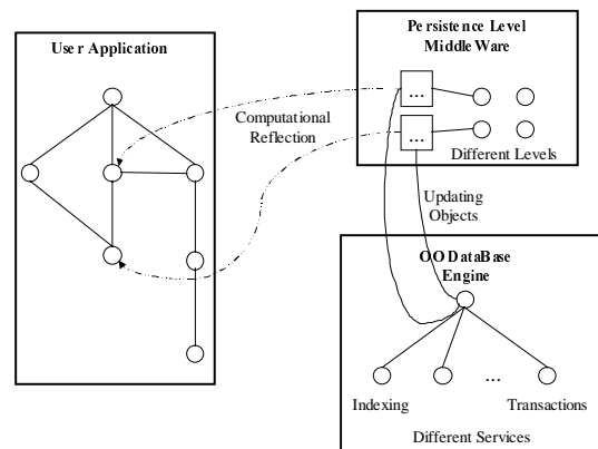
Figure 5 Overall structure of an implicit persistence reflective system
