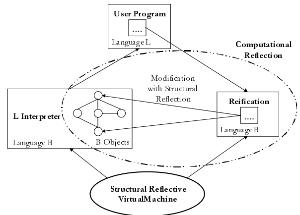
Figure 4 Computational reflection on an abstract machine with structural reflection
